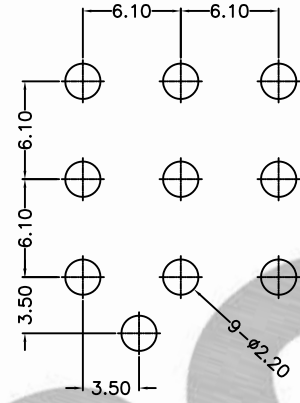
Panel Layout
